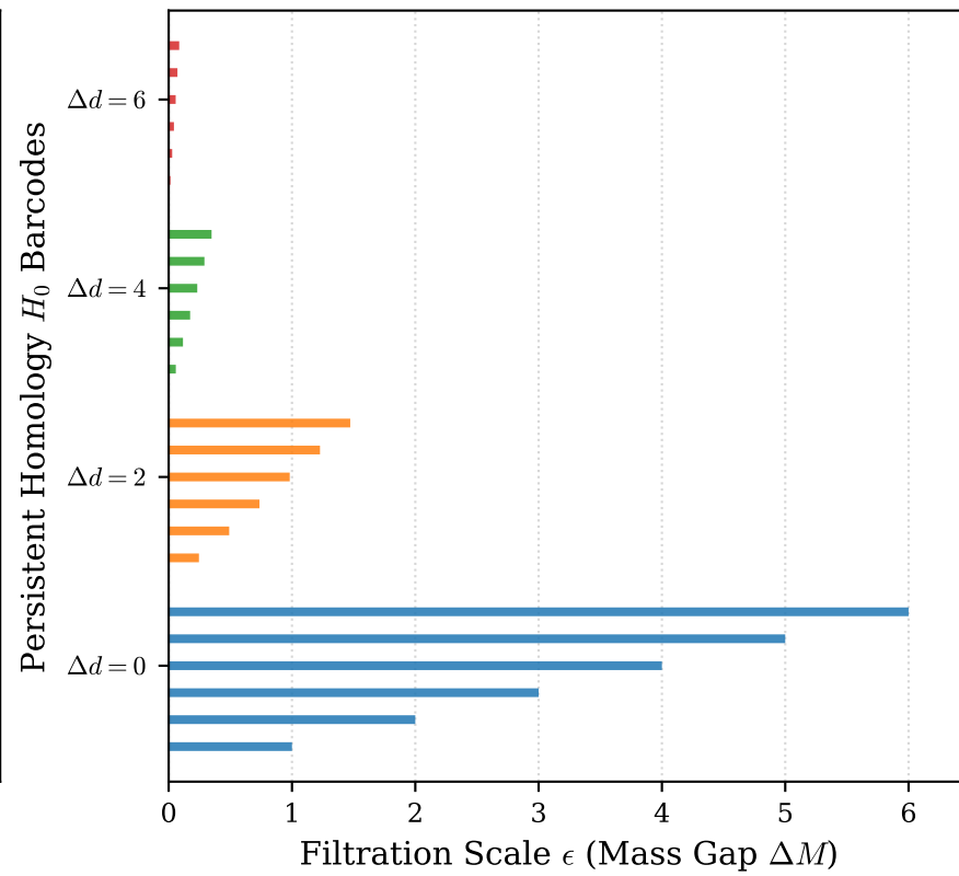
(e) CDL Bounce Instanton ( S_E = 316.0 )
