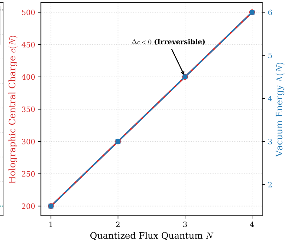
(f) Holographic c -Theorem Across Flux Decay
